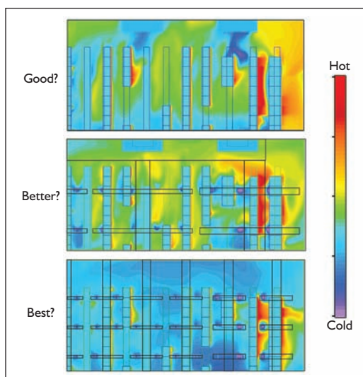
Figure 1: Temperature CFD data for three equipment environments (plan view).
