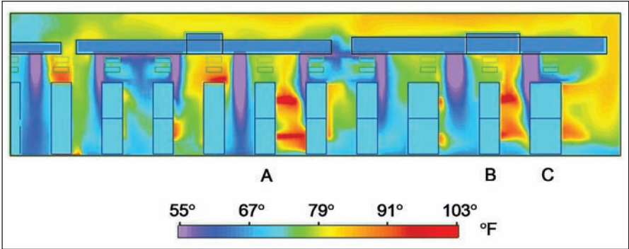
Figure 2: Point loads on perimeter aisle, lineup C (section view).
