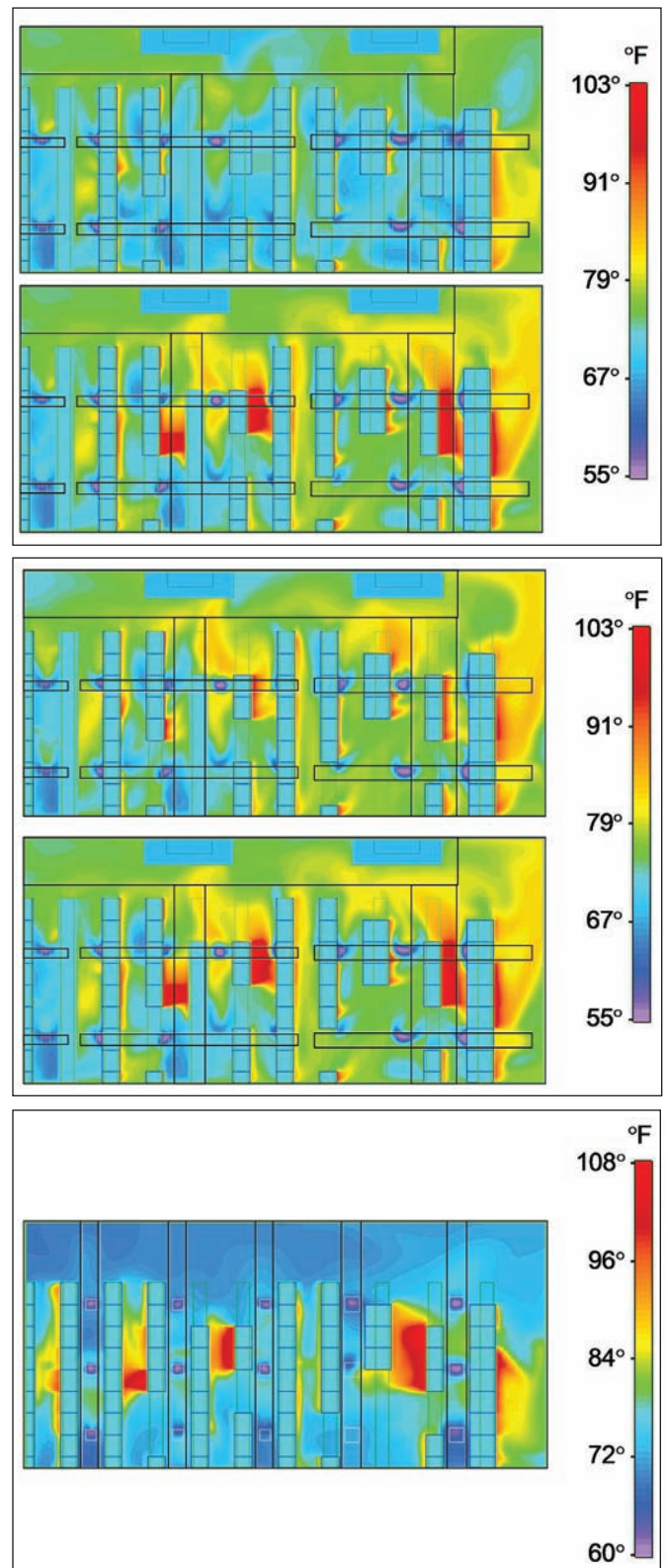
Figure 3 (top): With ( RCI_{HI} = 100\% ) and without ( RCI_{HI} = 95\% ) rear-door heat exchangers (plan view). Figure 4 (middle): With ( RCI_{HI} = 99\% ) and without ( RCI_{HI} = 95\% ) exhaust deflection devices (plan view). Figure 5 (bottom): Organized front-to-front ( RCI_{HI} = 99\% ) layout (plan view).
